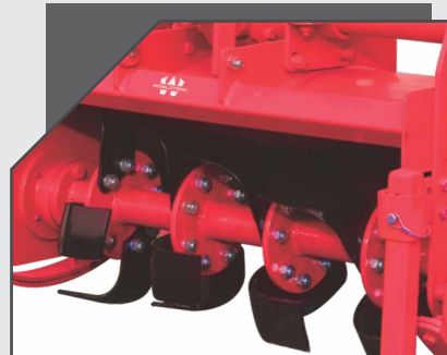
BORON STEEL BLADES WITH HELICAL ROTOR DESIGN
