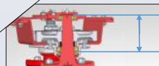
Optimum clearance between Rotor bearings for more stability
